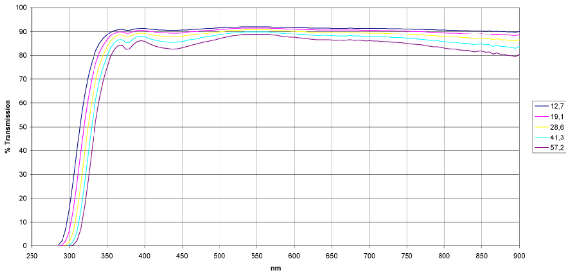
SUPREMAX ® glass – transmission for different glass thickness
